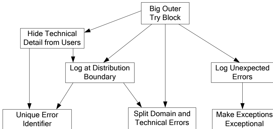
Figure 1 - Error Handling Patterns
