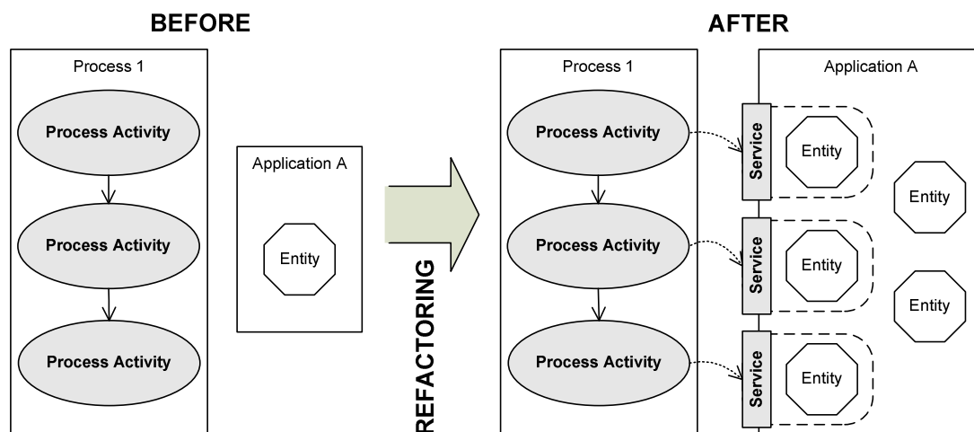
Figure 3: Refactoring by restructuring a application-specific business object model
