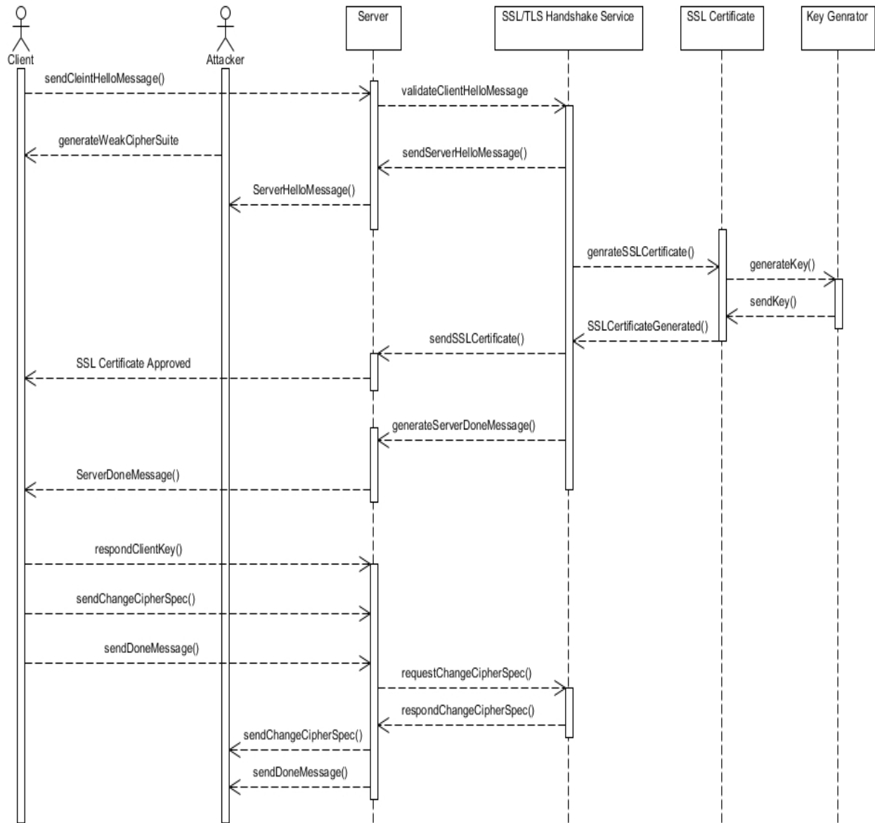
Fig. 4. Cipher Suite Rollback Attack Sequence Diagram
