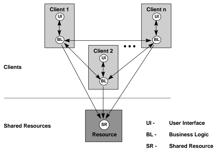
Figure 2: Client-side interconnection for access coordination
