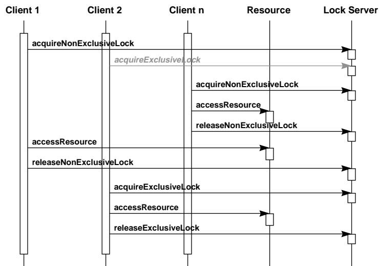
Figure 4: Sample scenario showing lock acquisition
